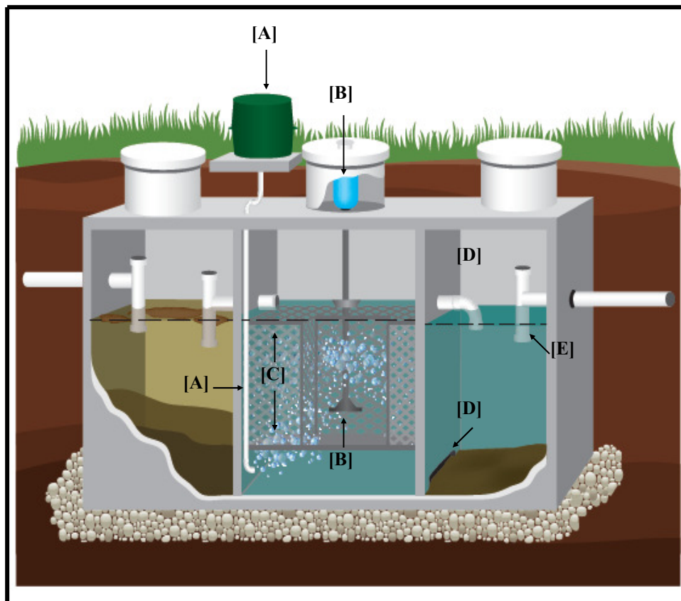
Figure 2: Aeration Treatment Unit (ATU). Many manufacturers and models of ATUs comply with the requirements of NSF Standard 40. Different models use different parts and methods to treat WASTEWATER to be in compliance with this standard.
